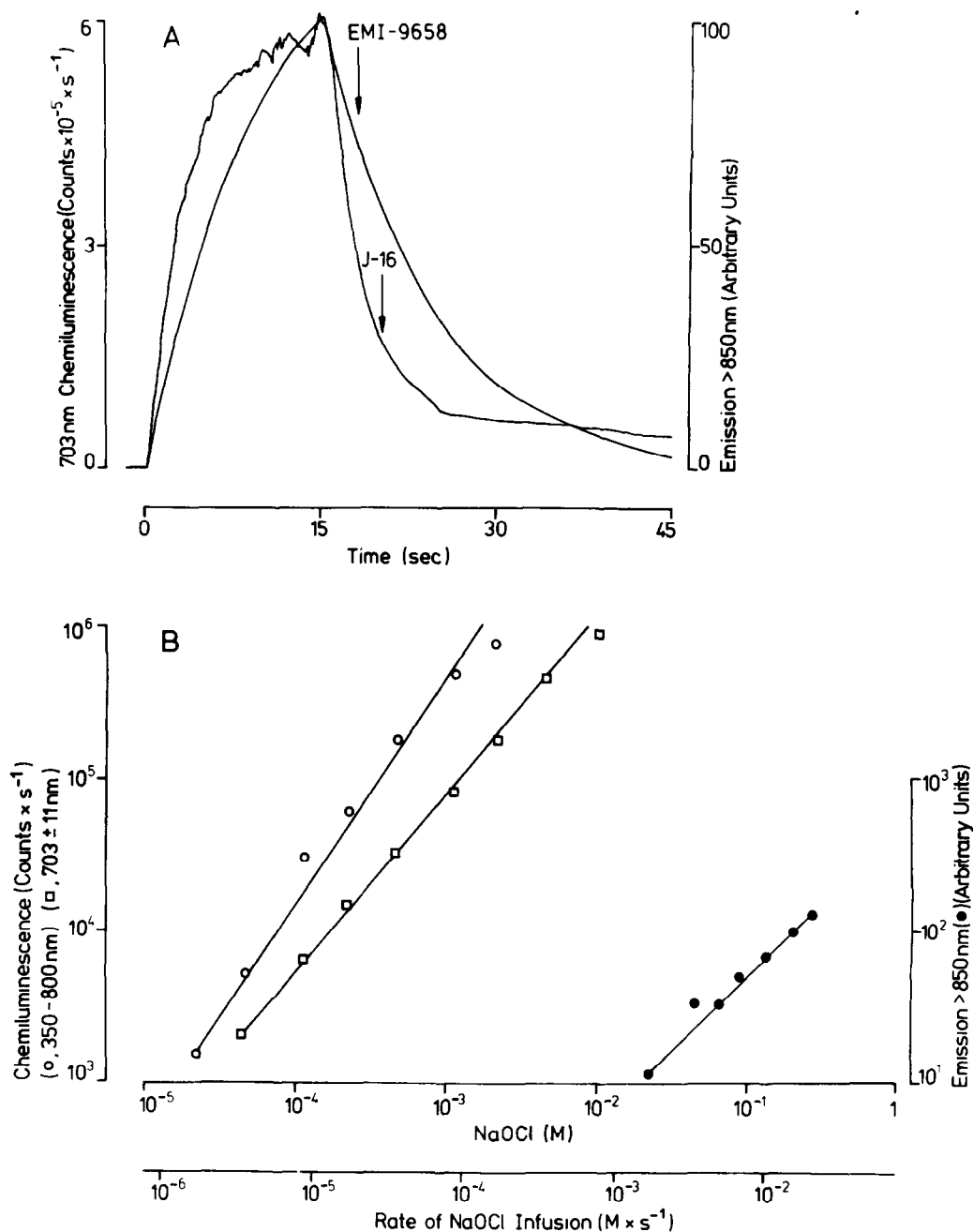
Fig.1. Monomol and dimol emission from the \text{H}_2\text{O}_2\text{-OCI}^- system. Assay conditions as described in section 2. (A) Time course of light emission arising from the \text{H}_2\text{O}_2\text{-OCI}^- system as detected by the red-sensitive photomultiplier (0.6 M NaOCl infused at a rate of 9.2 \mu\text{l} \cdot \text{s}^{-1} into 7 ml 1.8 M aqueous solution of \text{H}_2\text{O}_2 ) and the germanium diode (0.6 M NaOCl infused at a rate of 45 \mu\text{l} \cdot \text{s}^{-1} into 2.0 ml of 1.8 M \text{H}_2\text{O}_2 ). (B) Comparison of sensitivity of the employed red-sensitive photomultiplier (○, □) and germanium diode (●) for the \text{H}_2\text{O}_2\text{-OCI}^- chemiluminescence reaction. EMI-9658, photomultiplier; J-16, germanium diode.
