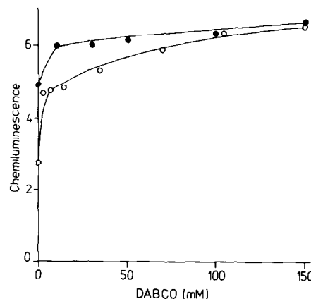
Fig.2. Enhancement of monomol and dimol emission by DABCO. Assay conditions: 0.6 M NaOCl was infused at a rate of 45\text{ }\mu\text{l}\cdot\text{s}^{-1} and 3.6\text{ }\mu\text{l}\cdot\text{s}^{-1} for monomol and dimol emission experiments, respectively, in the presence of increasing concentrations of DABCO. Values in the y-axis indicate 703 nm emission (○) detected by the red-sensitive photomultiplier expressed in \text{counts}\cdot\text{s}^{-1}\times 10^{-5} ; (●) 1274 nm chemiluminescence expressed in arbitrary units.
