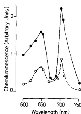
Fig.3. Spectral analysis of red-band chemiluminescence from the H_2O_2\text{--}OCl^- system in the absence (○) and presence (●) of DABCO. NaOCl was infused at a rate of 3.6\text{ }\mu\text{l}\cdot\text{s}^{-1} during 15 s (total NaOCl infused 4.7 mM) into 7.0 ml of 1.8 M H_2O_2 . DABCO, when present, 100 mM. Values are corrected for spectral response of the photomultiplier and spectral characteristics of the filters.
